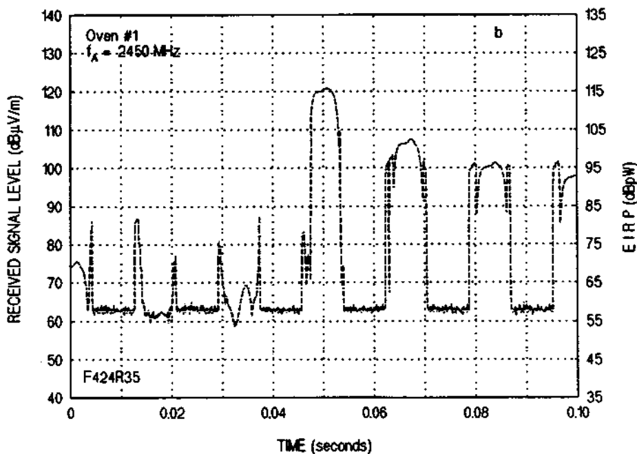
Figure 5-5b. Oven #1, Time vs. Amplitude at 2450 MHz.
