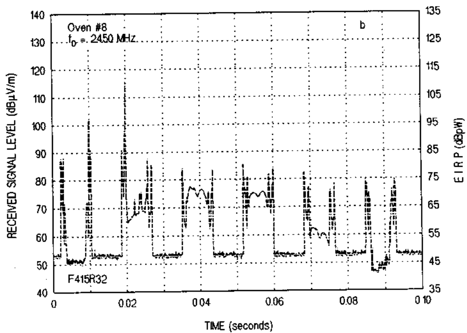
Figure 5-8b. Oven #8, Time vs. Amplitude at 2450 MHz.
