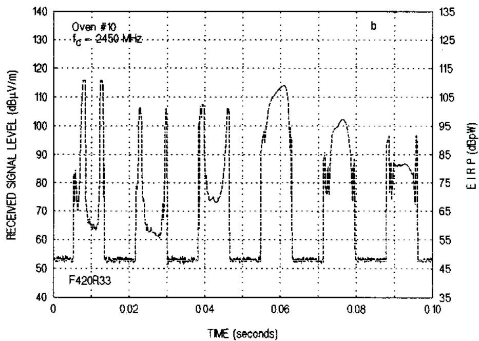
Figure 5-7b. Oven #10, Time vs. Amplitude at 2450 MHz.
