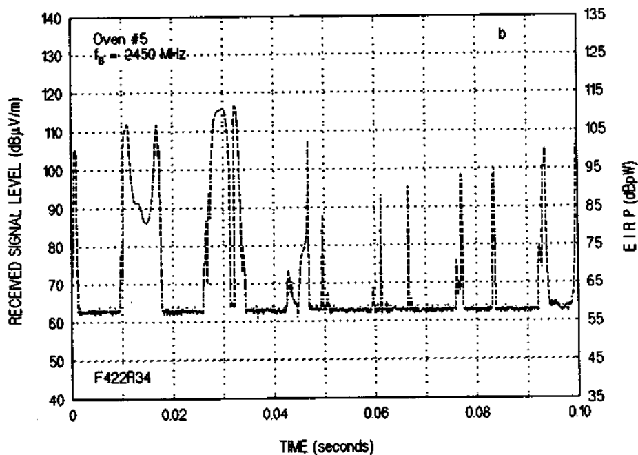
Figure 5-6b. Oven #5, Time vs. Amplitude at 2450 MHz.
