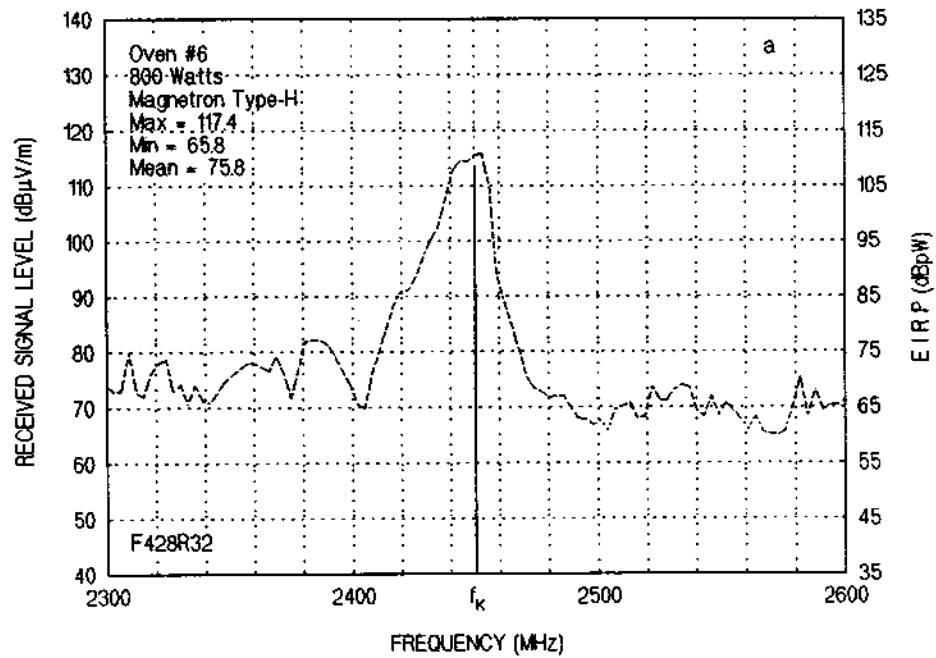
Figure 5-16a. Oven #6, Frequency vs. Amplitude.
