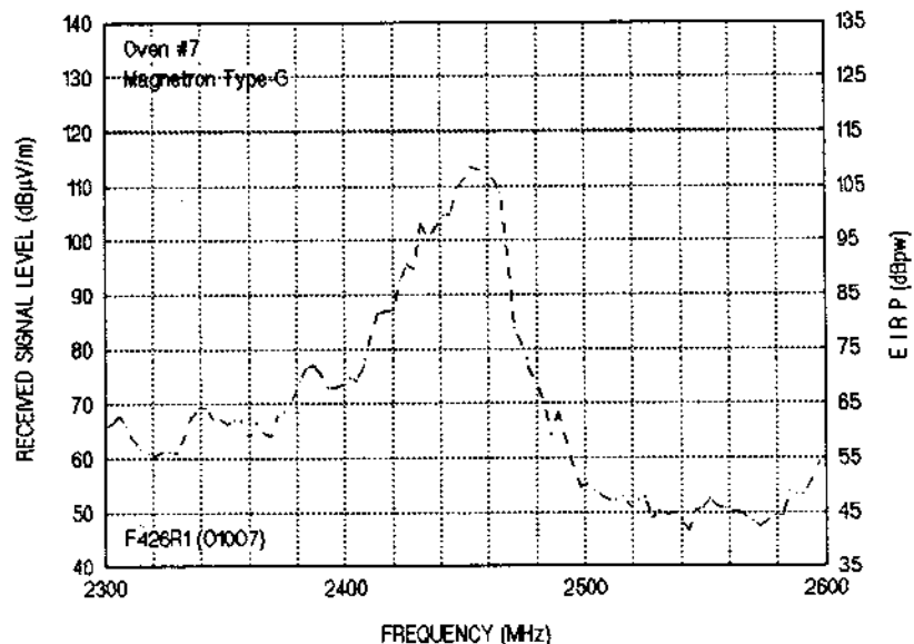
Figure 5-21. Frequency vs. Amplitude for Oven #7.
