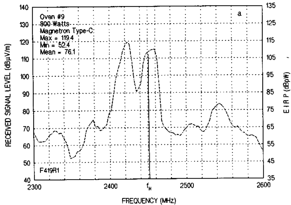
Figure 5-11a. Oven #9, Frequency vs. Amplitude.
