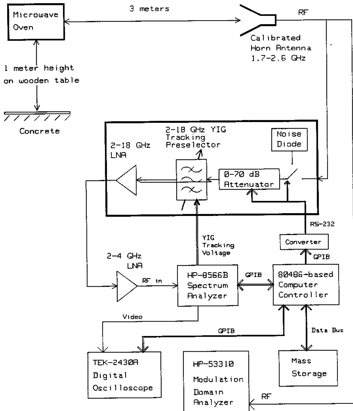
Figure 3-1. Measurement configuration.
